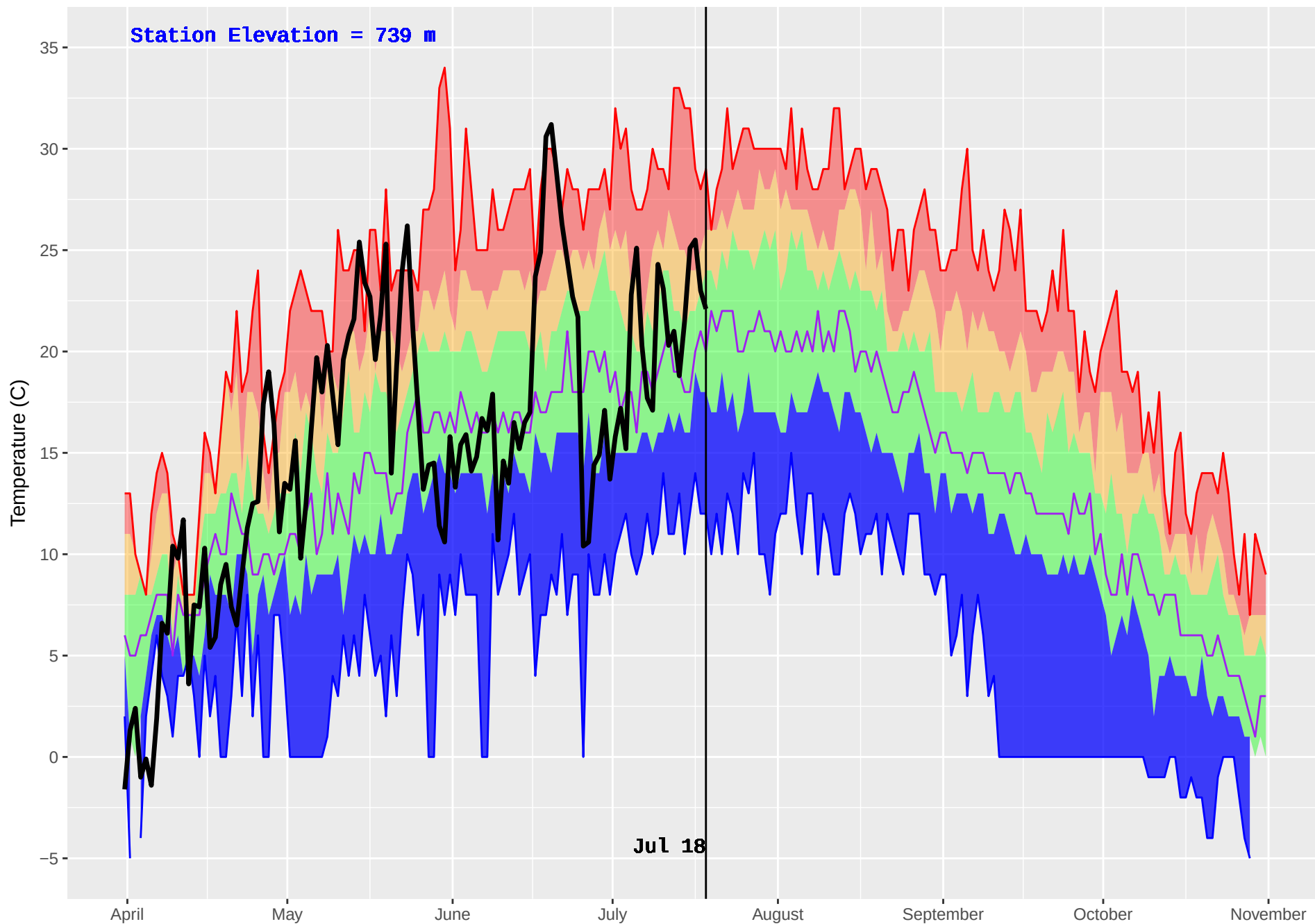
BEAR LAKE (149) : Historical (1980–2016) and Current (2018) Daily Temperature
