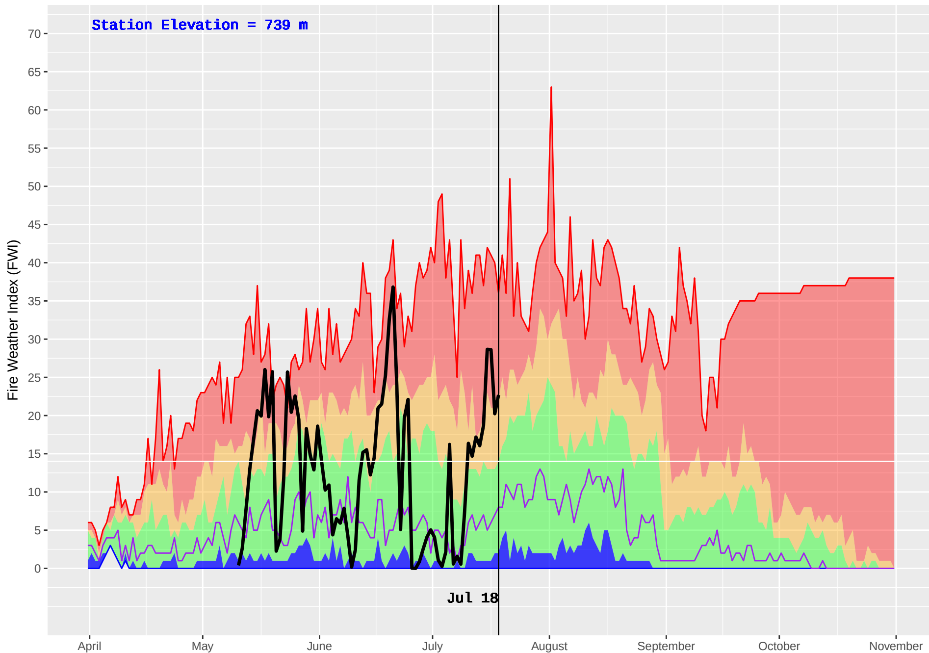
BEAR LAKE (149) : Historical (1980–2016) and Current (2018) Daily Fire Weather Index (FWI)
